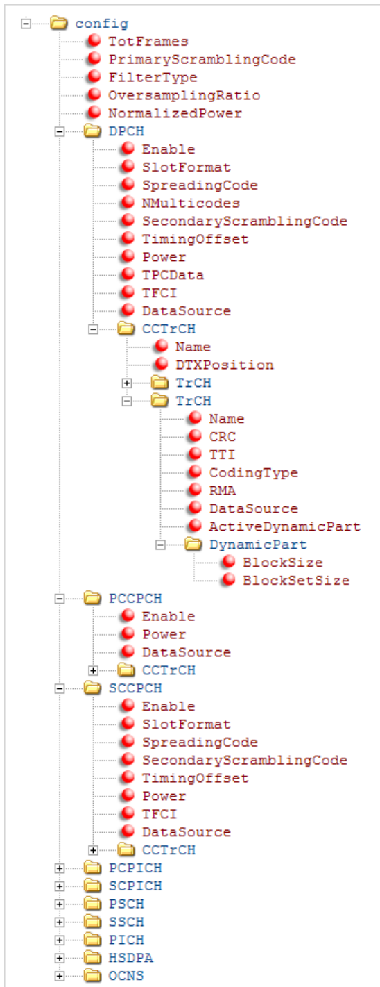
The config structure with DPCH, CCTrCH
