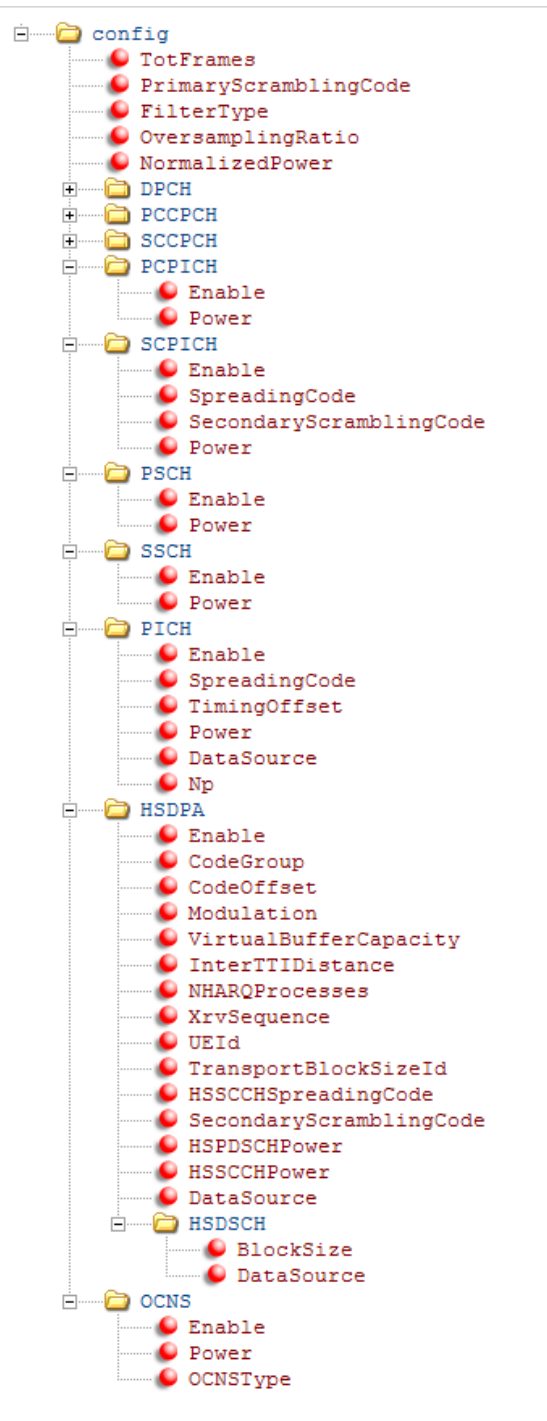
The config structure with PCPICH
